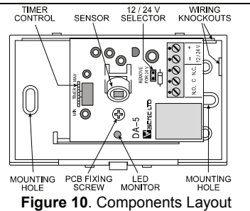
Figure 10. Components Layout
